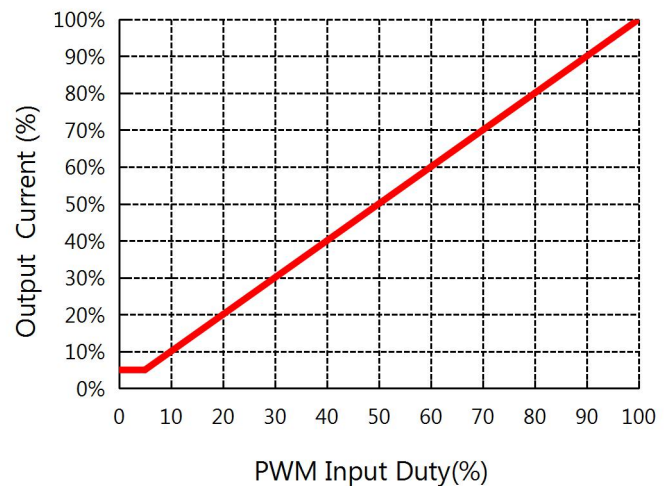
Fig. 8 PWM Dimming Curve
